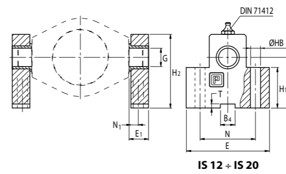
IS 12 + IS 20
