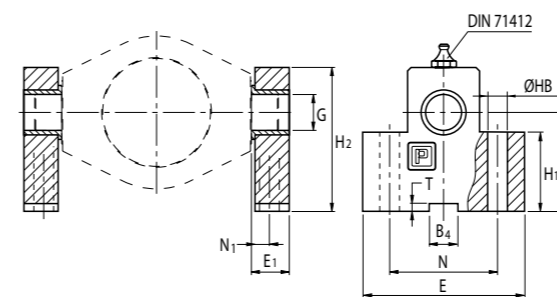
ISS 12 + ISS 20
